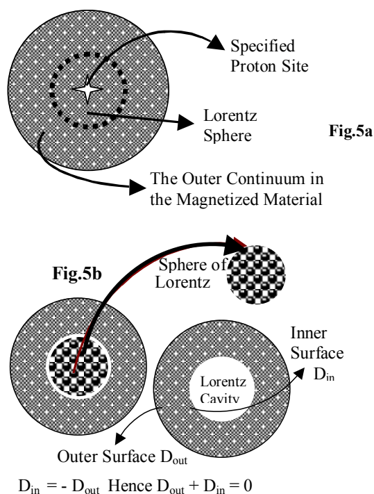
Fig.5 The various demarcations required, in an Organic Molecular Single Crystalline Spherical specimen, to Calculate the Contributions to the induced Fields at the specified site. D_{out/in} values stand for the corresponding Demagnetization Factors
